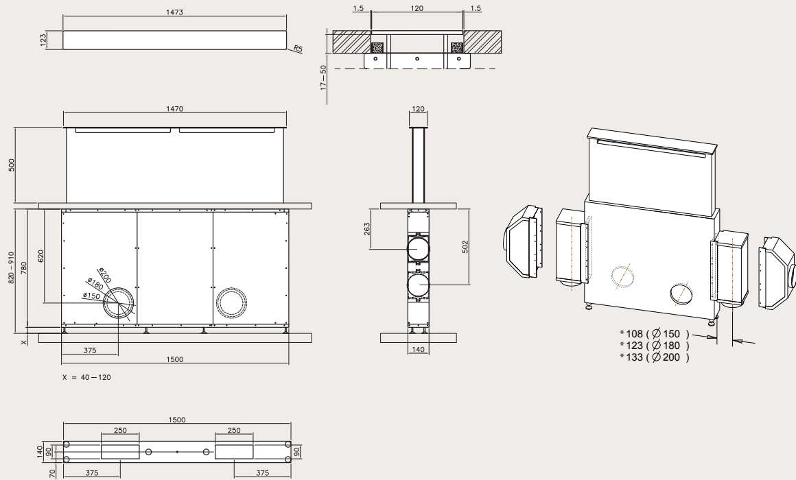
Transition piece
